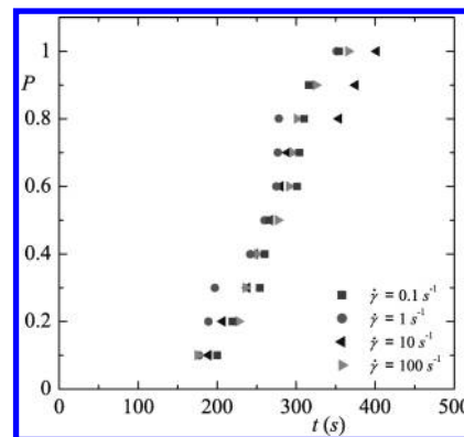
Figure 5. Critical time probability for the CP emulsion as a function of time for T = -6.3 \pm 0.5 \text{ }^\circ\text{C} (266.85 K) and for 4 different shear rate values \dot{\gamma} = 0.1, 1, 10, \text{ and } 100 \text{ s}^{-1} .
